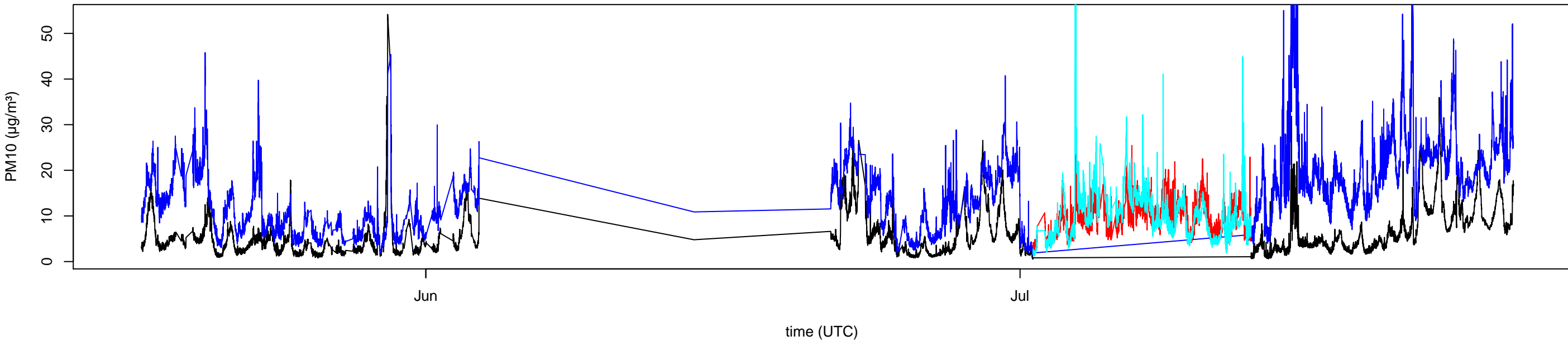
SDS011 660436 PM10 calibration(blue)/validation(red) data
