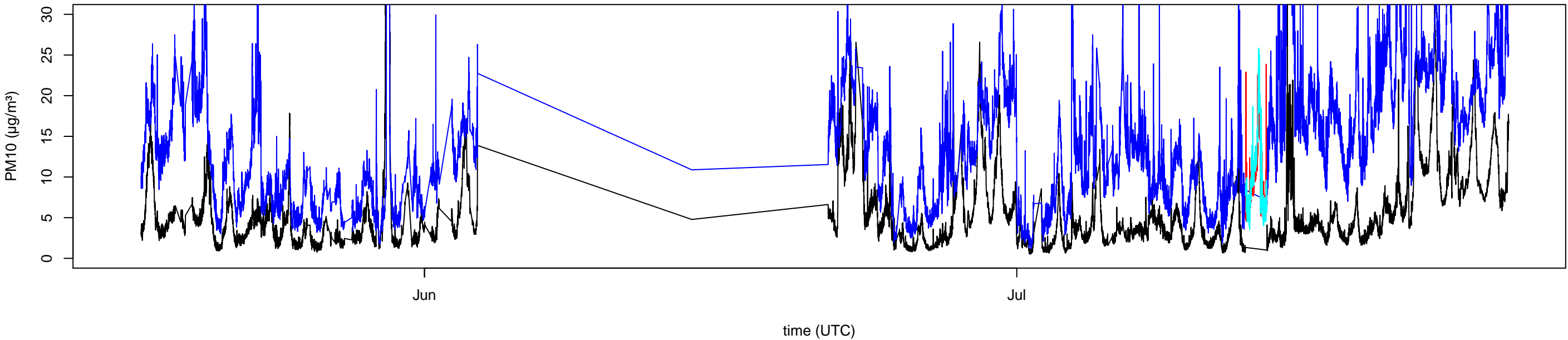
SDS011 660436 recalibrated PM10 data
