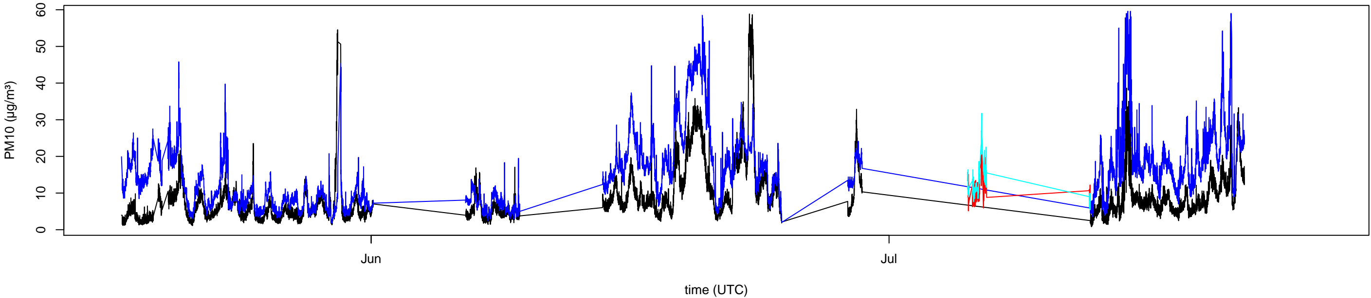
SDS011 5682100 PM10 calibration(blue)/validation(red) data
