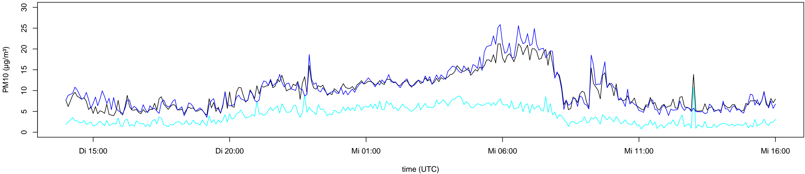
SDS011 550119 recalibrated PM10 data (black) 2022-07-12 14:00 to 2022-07-13 18:00 UTC
