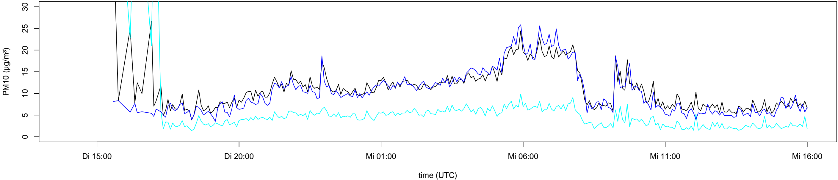
SDS011 2519718 recalibrated PM10 data (black) 2022-07-12 14:00 to 2022-07-13 18:00 UTC
