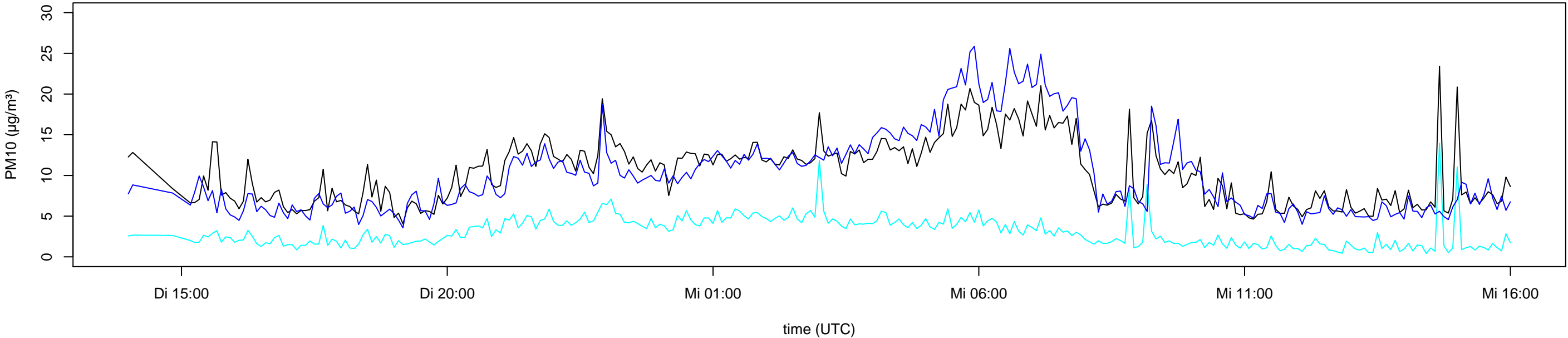
SDS011 14722068 recalibrated PM10 data (black) 2022-07-12 14:00 to 2022-07-13 18:00 UTC
