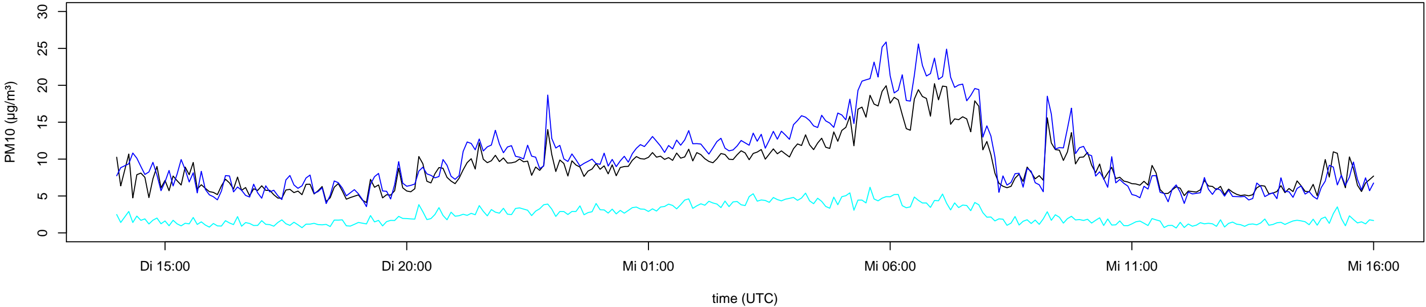
SDS011 14595225 recalibrated PM10 data (black) 2022-07-12 14:00 to 2022-07-13 18:00 UTC
