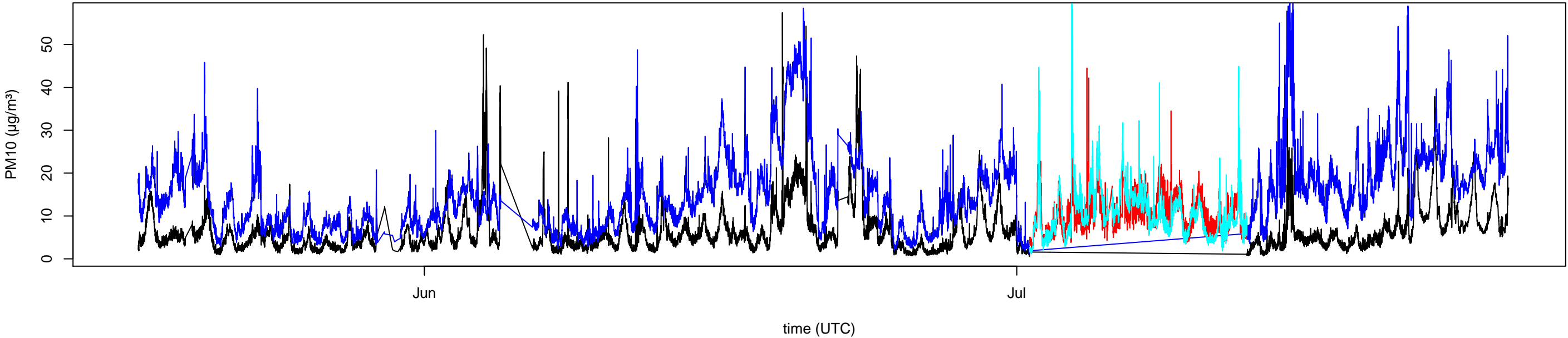
SDS011 14595225 PM10 calibration(blue)/validation(red) data
