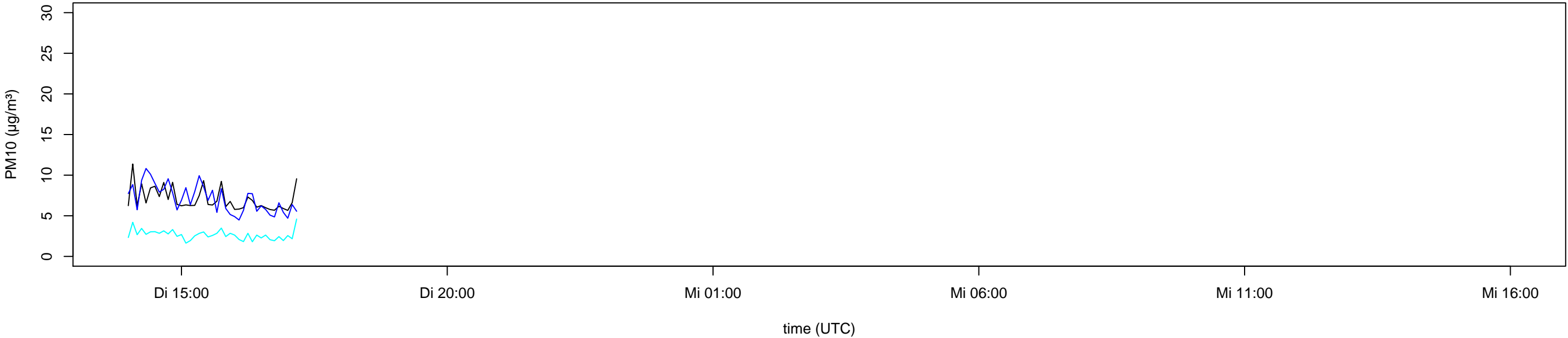
SDS011 14573303 recalibrated PM10 data (black) 2022-07-12 14:00 to 2022-07-13 18:00 UTC
