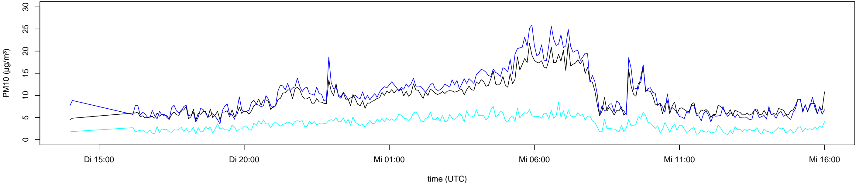
SDS011 14155848 recalibrated PM10 data (black) 2022-07-12 14:00 to 2022-07-13 18:00 UTC
