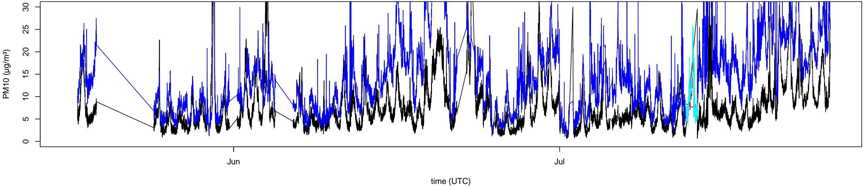
SDS011 14155848 recalibrated PM10 data
